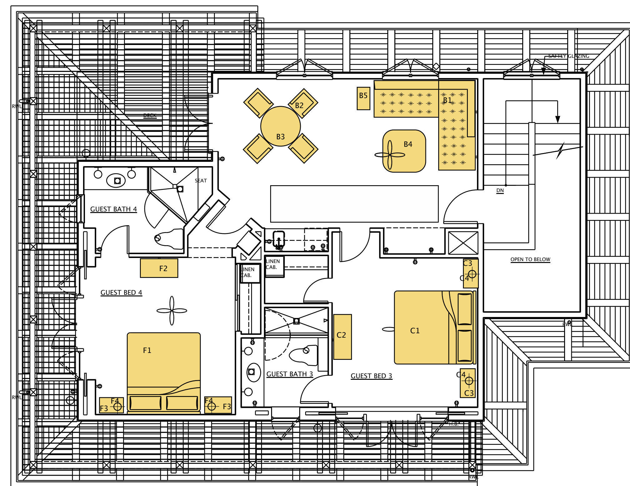
SECOND FLOOR GUEST WING
